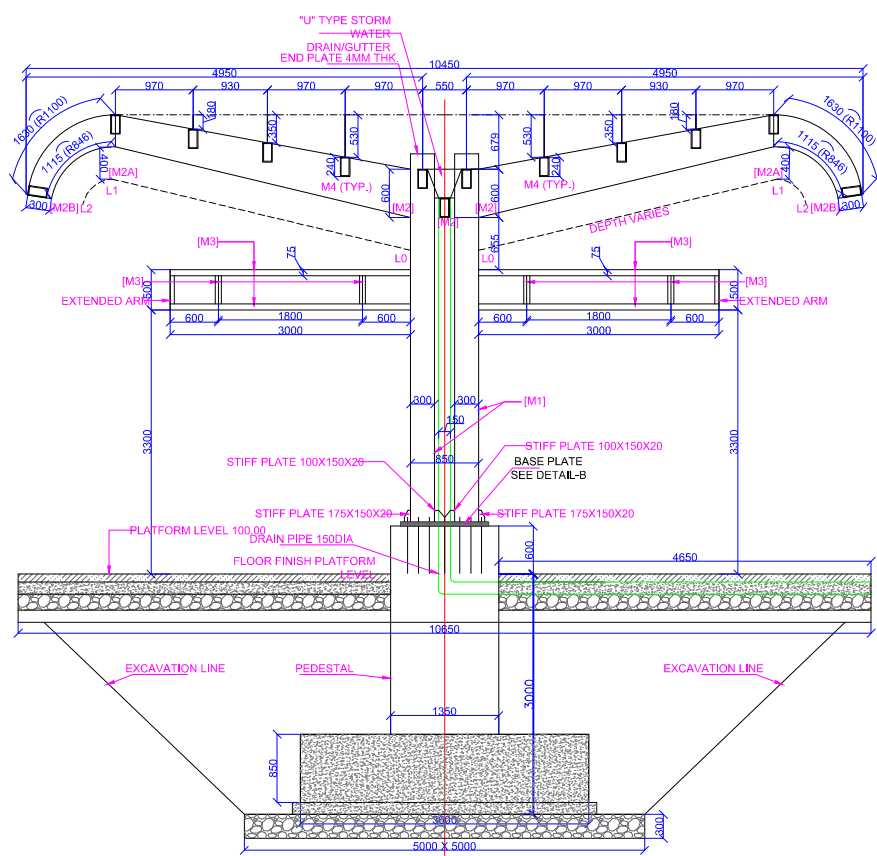
DESIGN C.O.P. SECTION FOR 12.00M SPAN WITH OUT O.H.E
