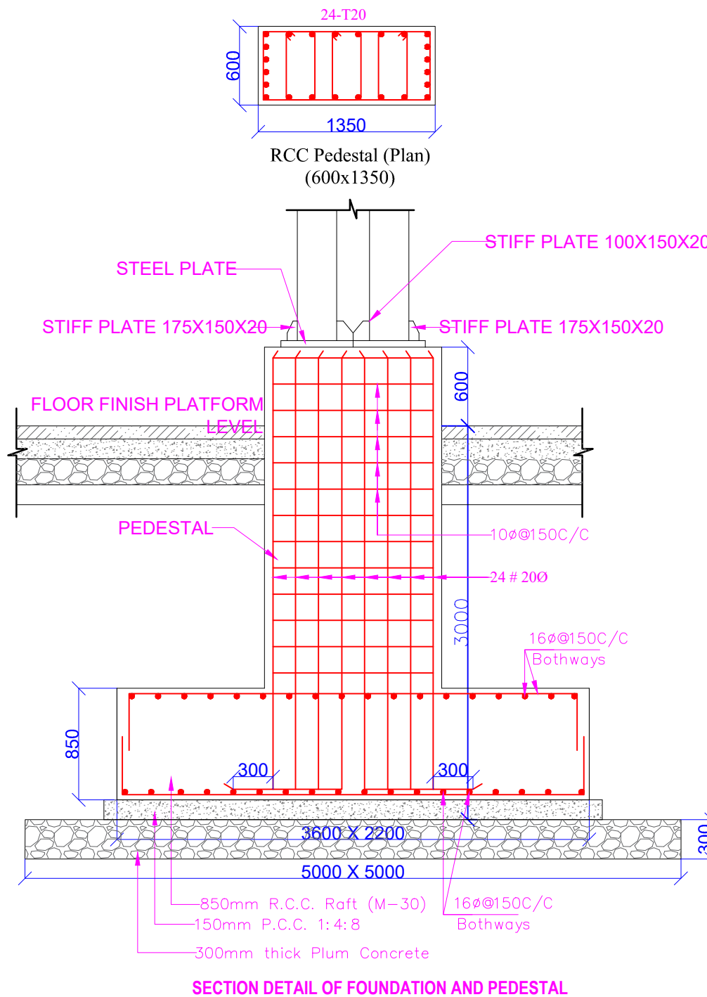
SECTION DETAIL OF FOUNDATION AND PEDESTAL
