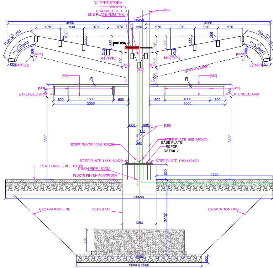
DESIGN C.O.P. SECTION FOR 12.00M SPAN WITH O.H.E
